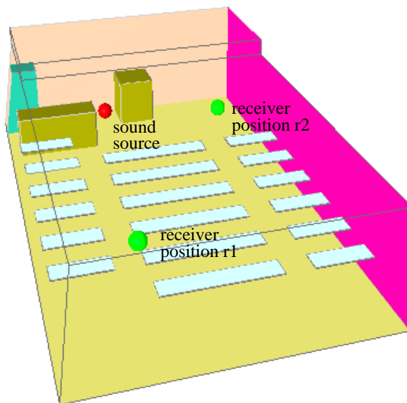
Figure 2: The 3D model of the studied lecture room. While recording binaural soundtracks the head was pointed to forward direction in recording positions r1 and r2. The height of the sound source was 1.2 m and the height of the recording positions were 1.7 m.
