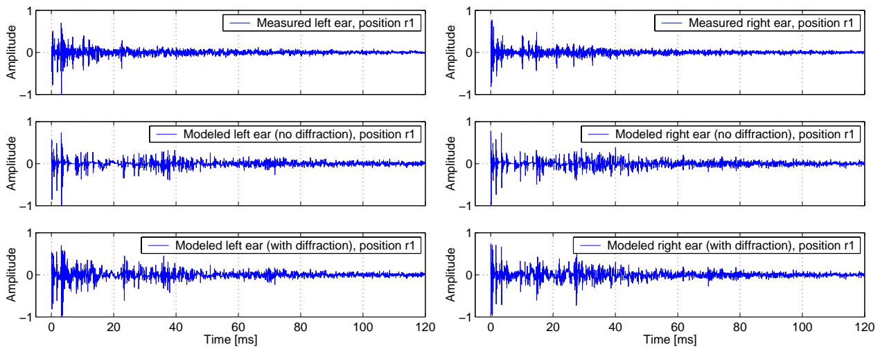
Figure 3: Modeled and measured binaural impulse responses at the listening position r1.
